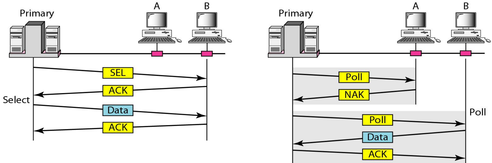
Figure 12.19 Select and poll functions in polling access method
