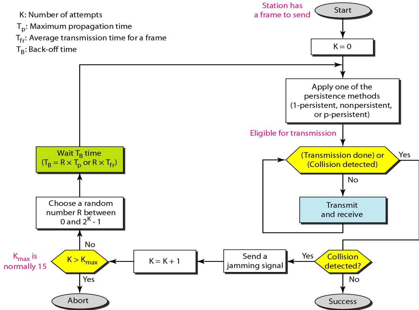
Figure 12.14 Flow diagram for the CSMA/CD
