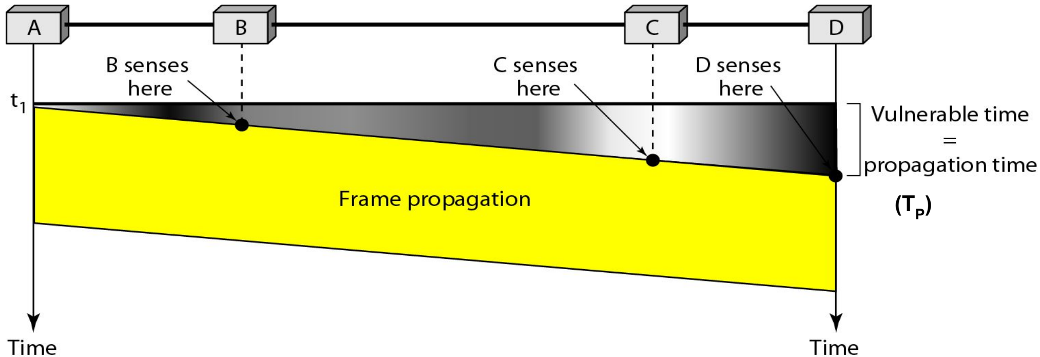
Figure 12.9 Vulnerable time in CSMA
